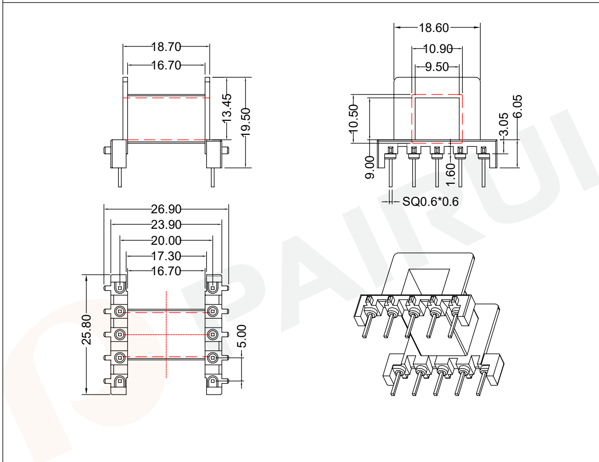
Winding data and area product for 10-pins EVD25 coil former
